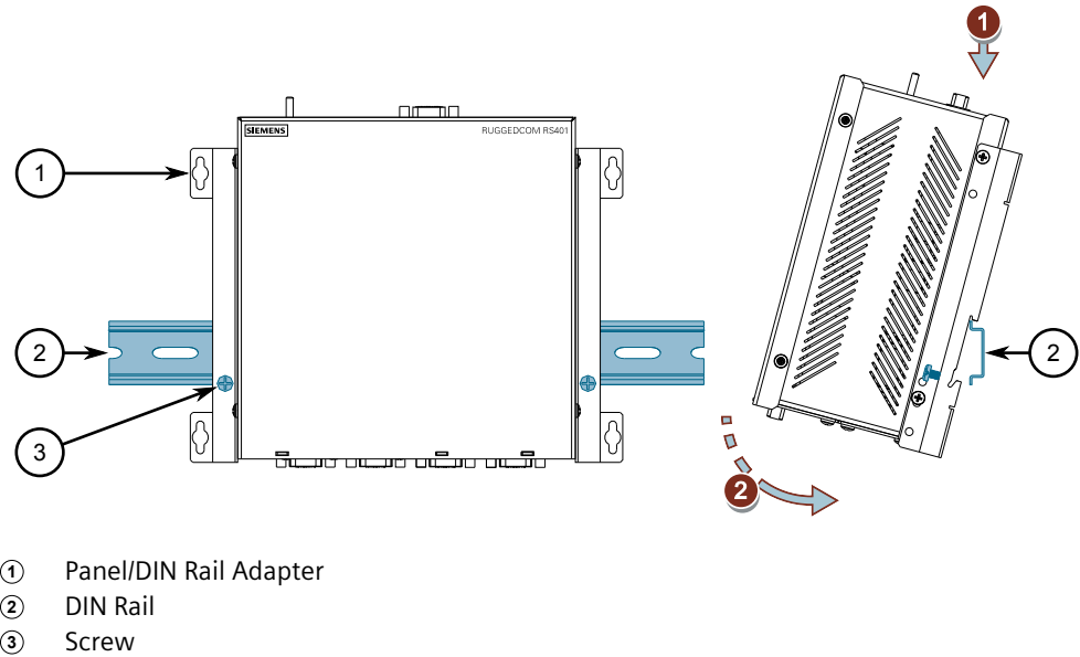
Figure 2.1 Mounting the Device to a DIN Rail (Front Panel Mount Option)
