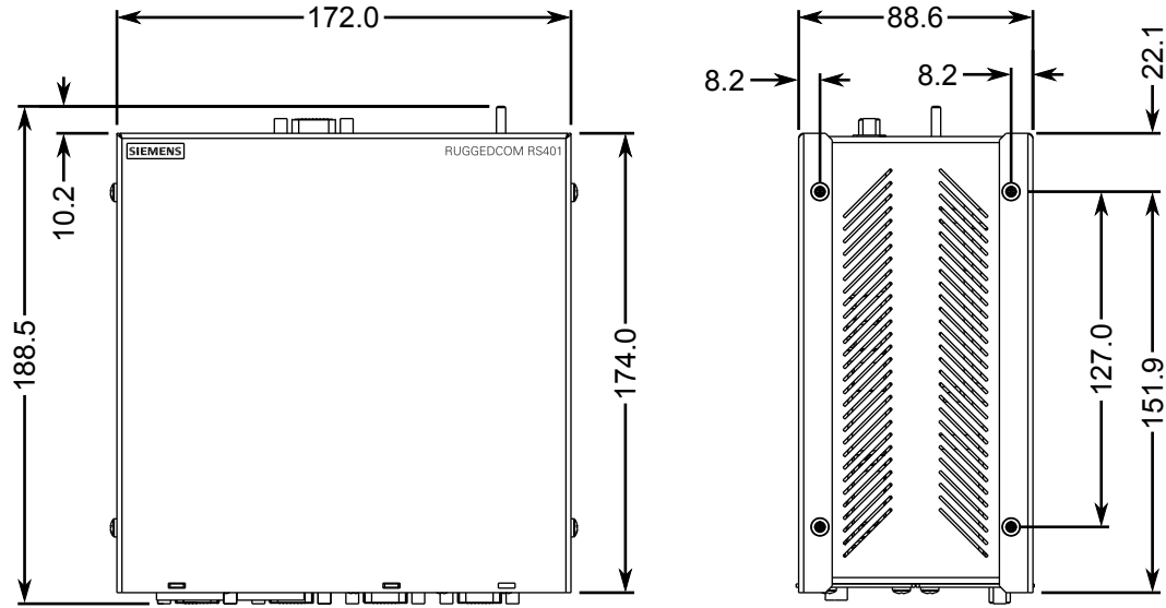
Figure 5.1 Overall Dimensions
