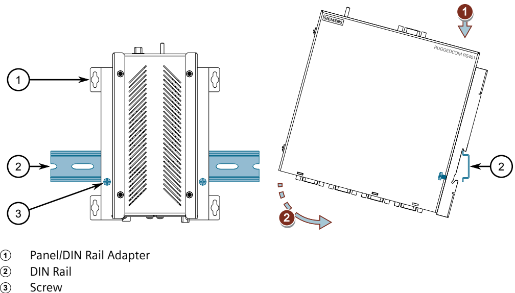
Figure 2.2 Mounting the Device to a DIN Rail (Side Panel Mount Option)
