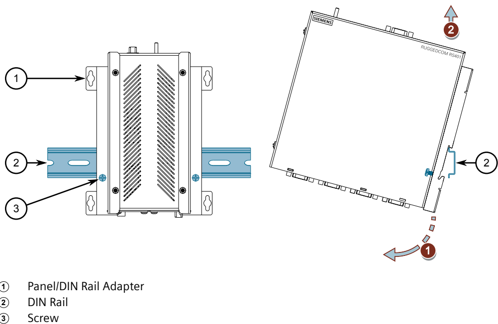
Figure 2.4 Removing the Device from a DIN Rail (Side Panel Mount Option)
