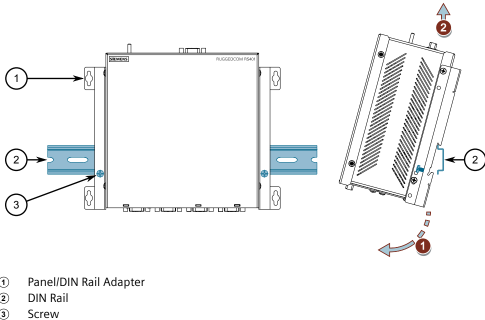
Figure 2.3 Removing the Device from a DIN Rail (Front Panel Mount Option)
