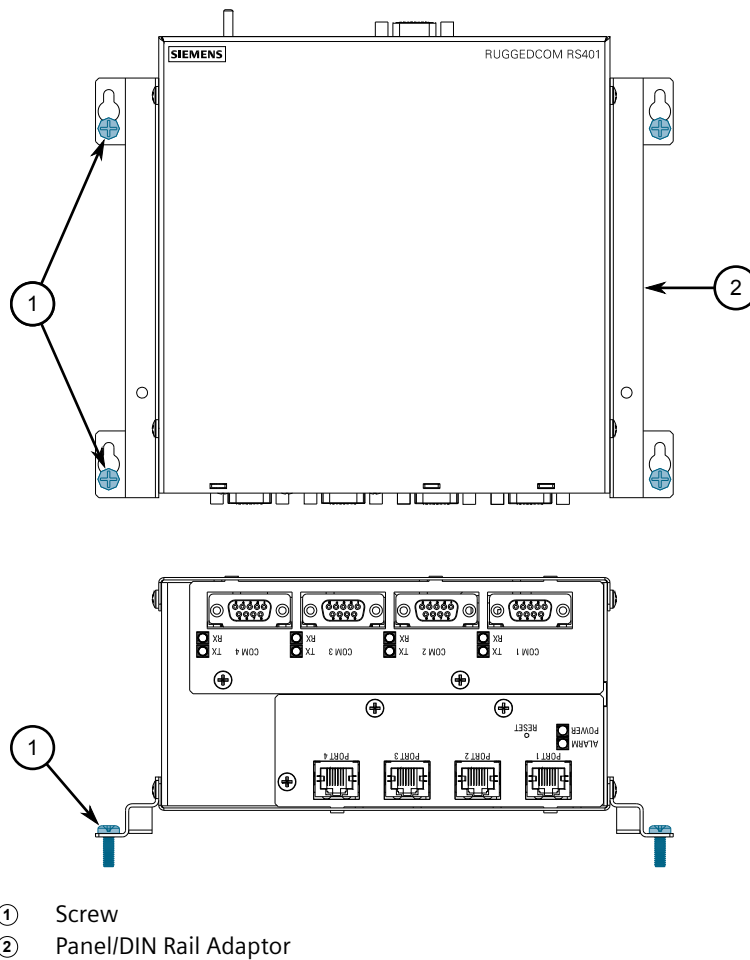
Figure 2.5 Panel Mounting (Front Mount Orientation)
