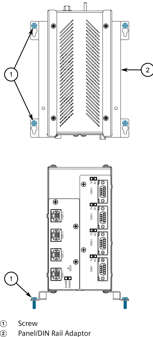
Figure 2.6 Panel Mounting (Side Mount Orientation)
