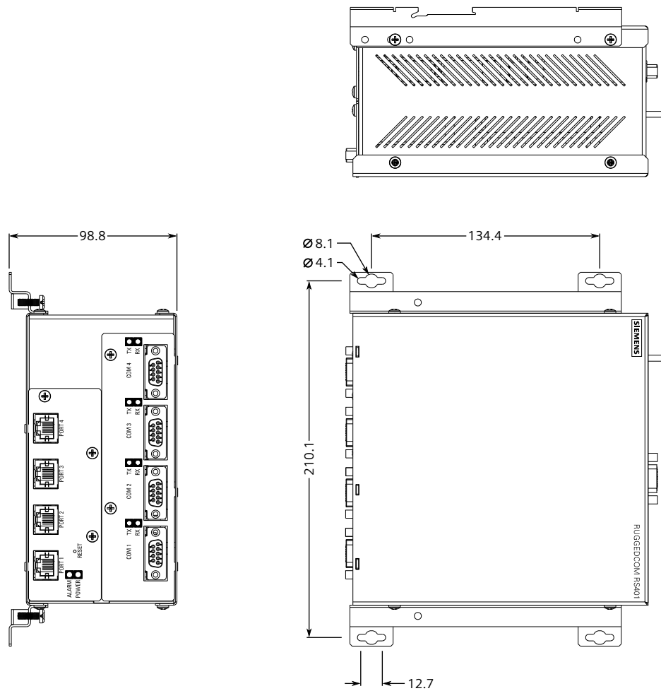
Figure 5.2 Panel and Din Rail Mount Dimensions (Front Mount Option)
