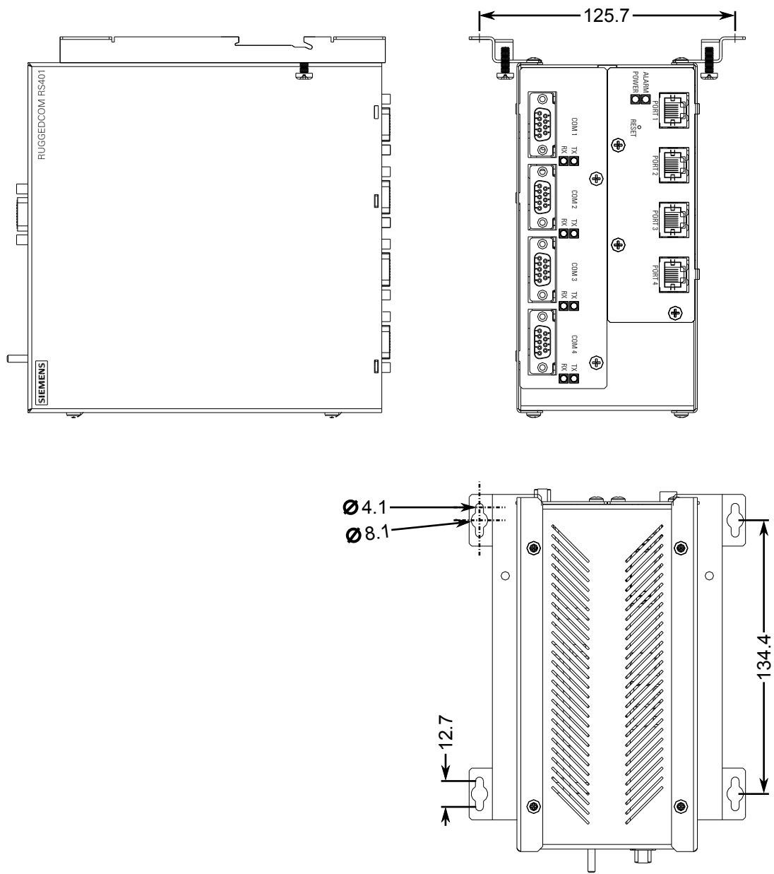
Figure 5.3 Panel and Din Rail Mount Dimensions (Side Mount Option)
